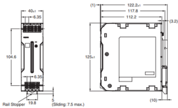
S8VK-T48024 (480 W)
