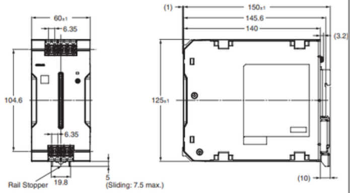
S8VK-T12424 (240 W)
