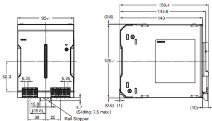
S8VK-T48024 (480 W)
